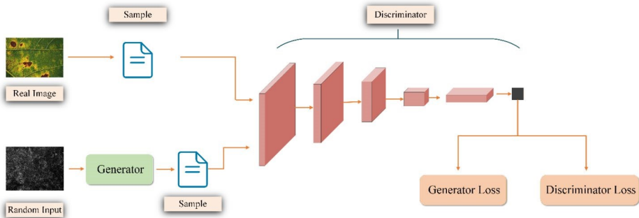
Fig. 9 Block Diagram of Generative Adversarial Networks (GAN) (Aggarwal et al. 2021)
